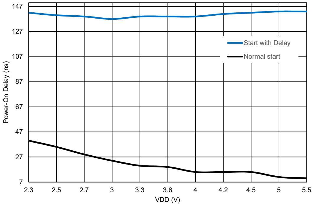
Figure 82: Oscillator2 Maximum Power-On Delay vs. V_{DD} at T = 25^{\circ}\text{C} , \text{OSC2} = 25\text{ MHz}
