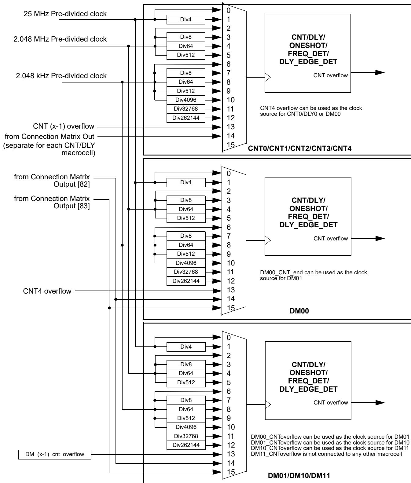
Figure 76: Clock Scheme
