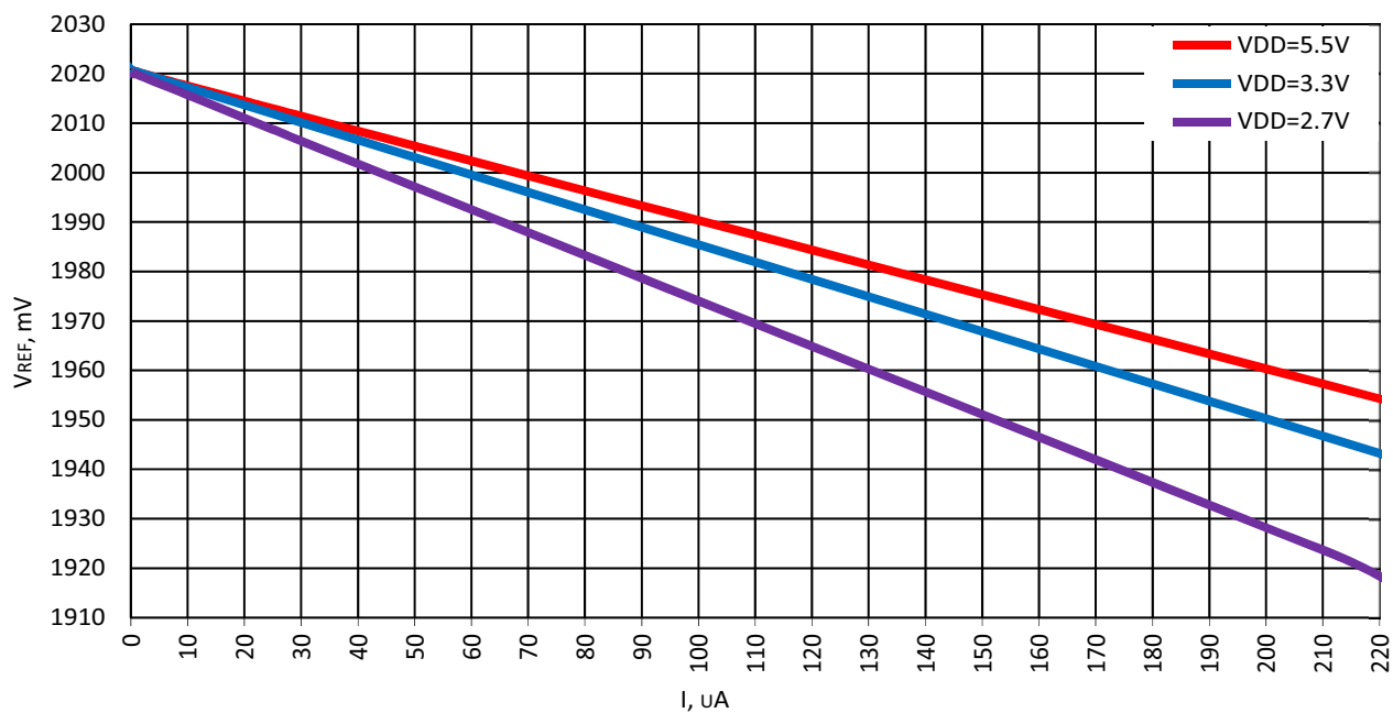
Figure 72: Typical Load Regulation, Vref = 2016 mV, T = -40 °C to +125 °C, Buffer - Enable
