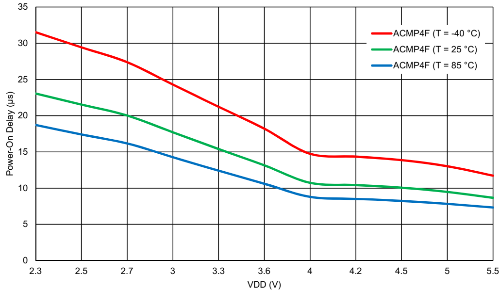
Figure 124: ACMP4F Power-On Delay vs. V_{DD}
