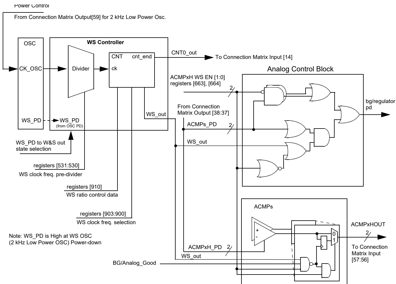
Figure 49: WS Controller
