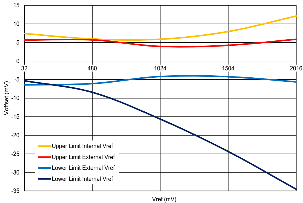
Figure 125: ACMP4F Input Offset Voltage vs. V_{ref} at T = -40\text{ °C} to 125\text{ °C} , Input Buffer Disabled
