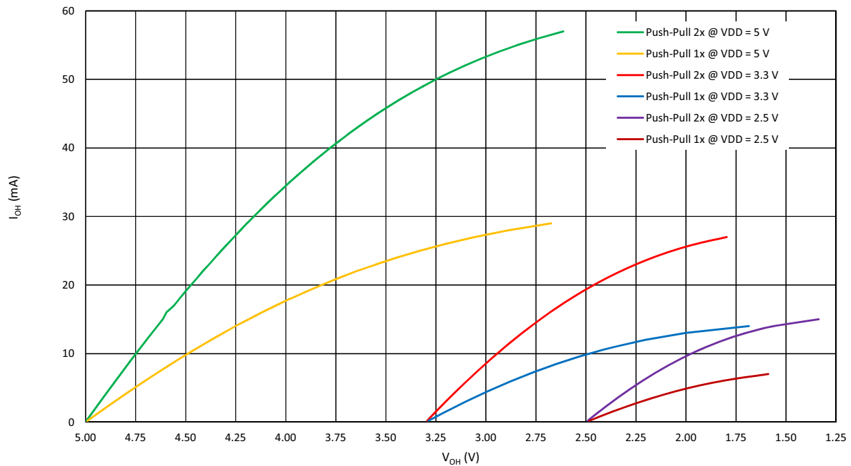
Figure 12: Typical High Level Output Current vs. High Level Output Voltage at T = 25^\circ\text{C}
