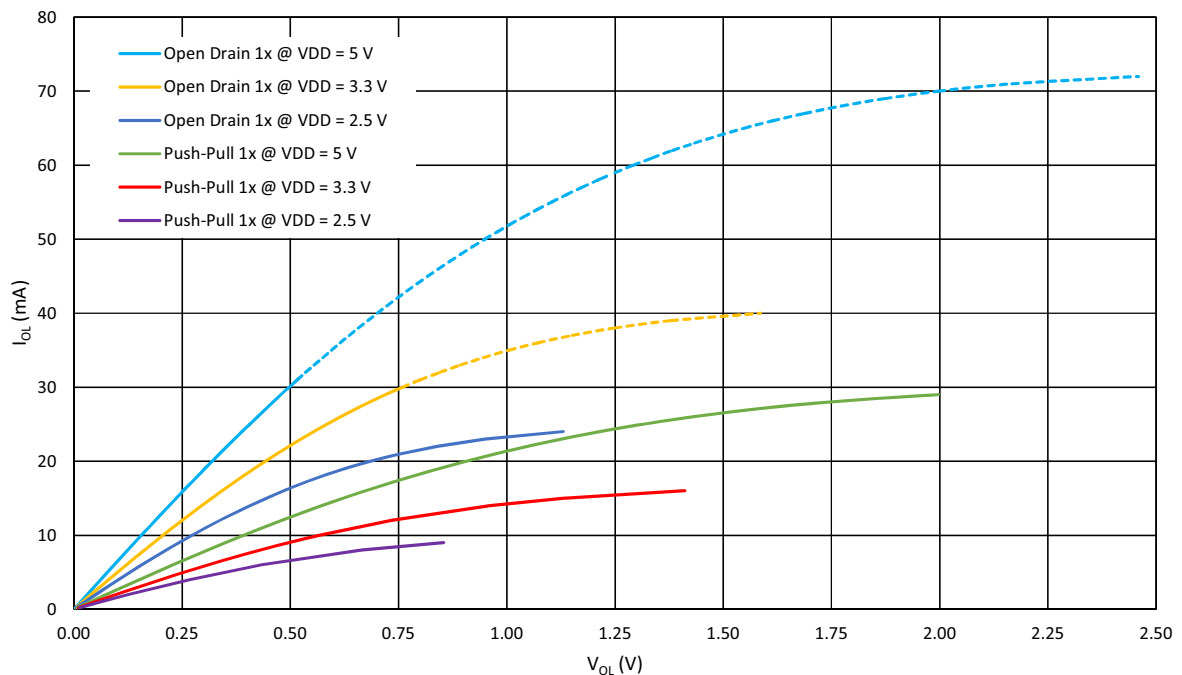
Figure 13: Typical Low Level Output Current vs. Low Level Output Voltage, 1x Drive at T = 25^\circ\text{C} , Full Range
