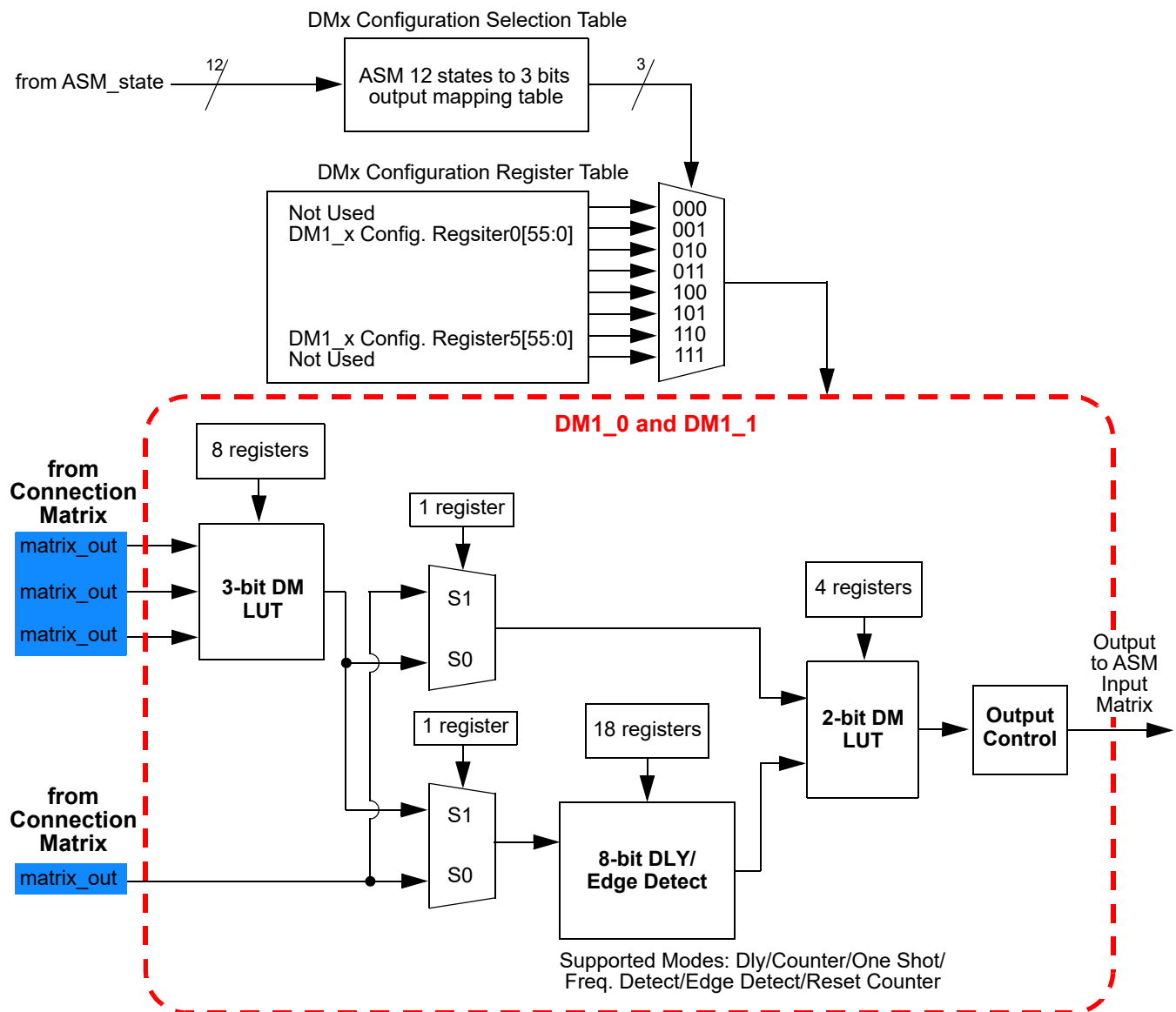
Figure 116: DM1_0/DM1_1 Inputs
