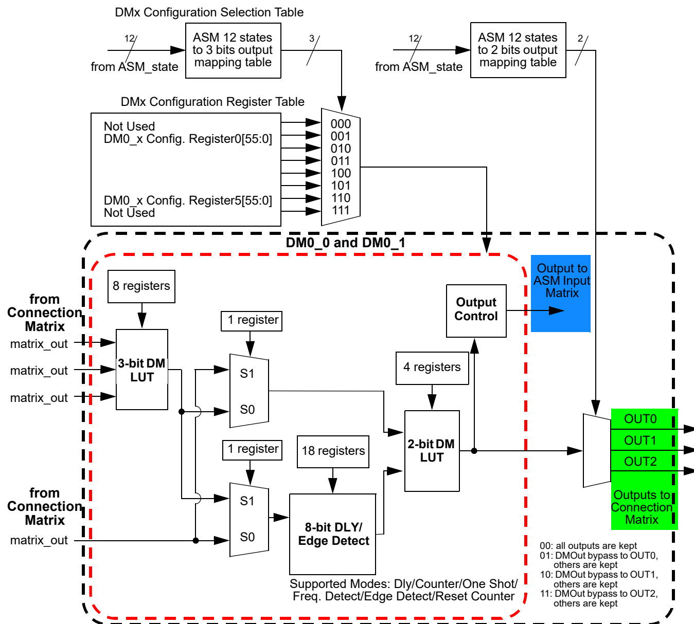
Figure 117: DM0_0/DM0_1 Outputs
