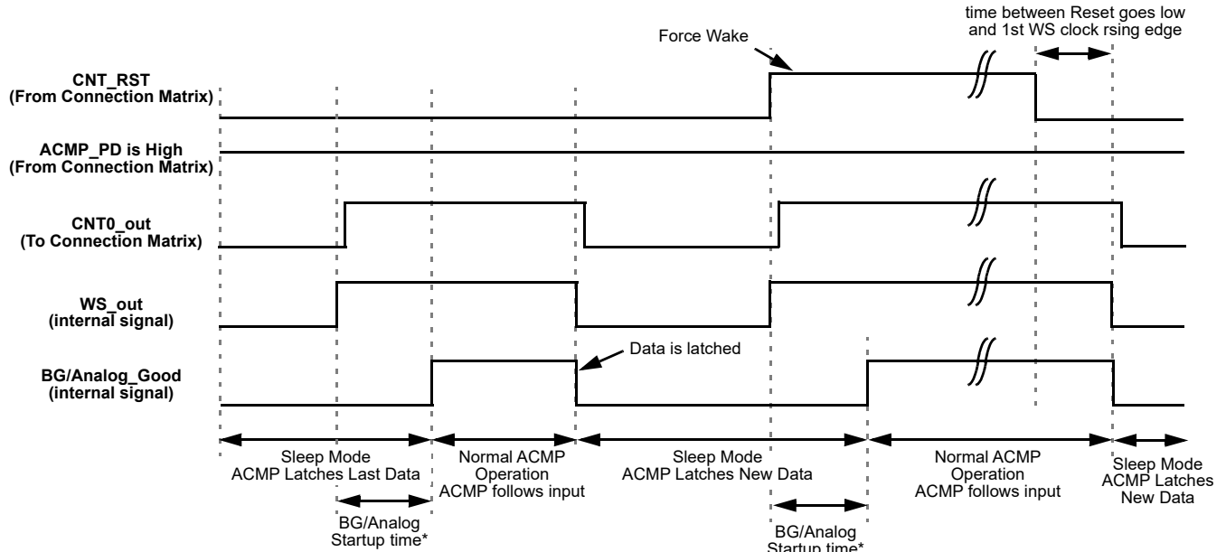
Figure 50: Wake/Sleep Timing Diagram, Normal Wake Mode, Counter Reset is Used
