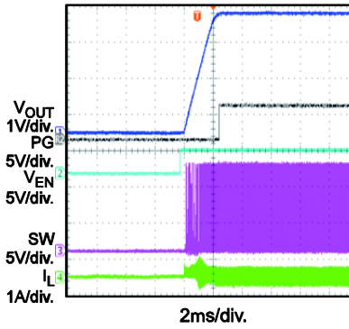
Start-Up through EN/SYNC I_{OUT}=0A
