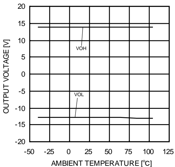
Figure 74. Maximum Output Voltage - Ambient Temperature ( V_{CC}/V_{EE}=+15V/-15V , R_L=2k\Omega )
