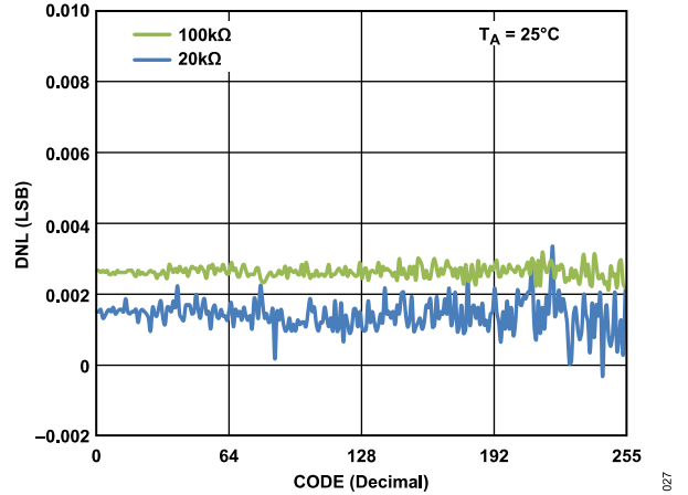
Figure 22. R-DNL in Normal Mode vs. Code vs. Nominal Resistance (AD5271)
