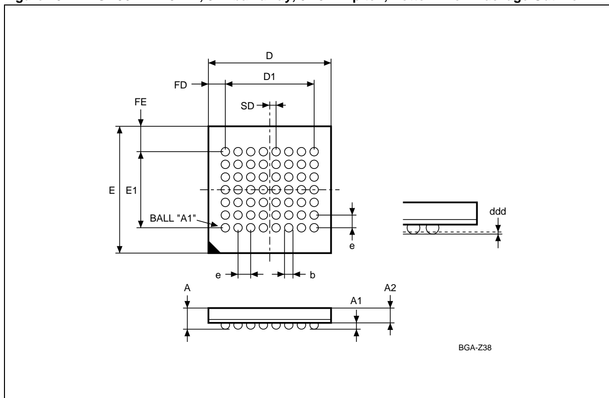
Figure 18. VFBGA56 - 7.7x9mm, 8x7 ball array, 0.75mm pitch, Bottom View Package Outline
