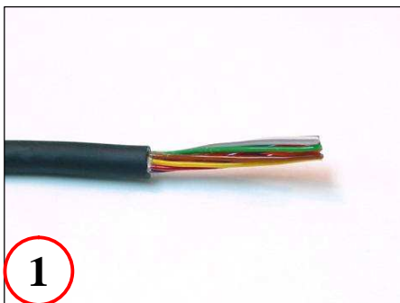
Strip off approximately 1 ¼ inch of cable jacket
