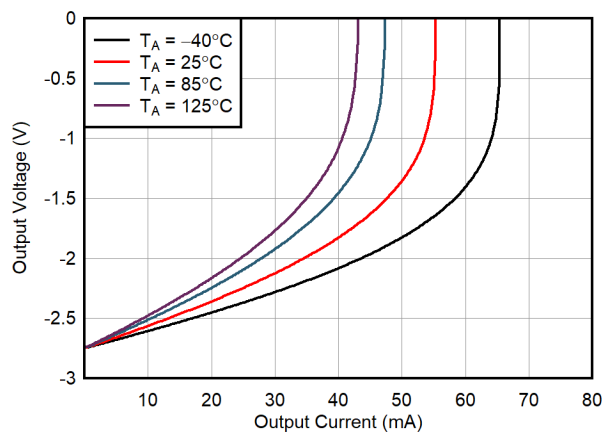
Figure 6-16. Output Voltage Swing vs Output Current (Sinking)
