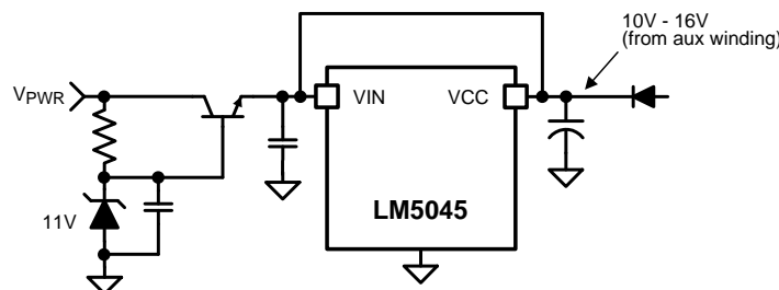
Figure 21. Start-Up Regulator For V_{PWR} > 100\text{ V}
