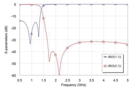
RFLPF10051G8DM5T51
