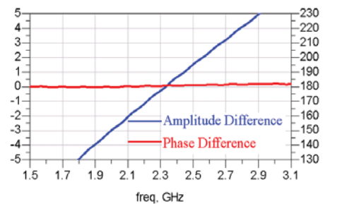
Amplitude and Phase Balance
