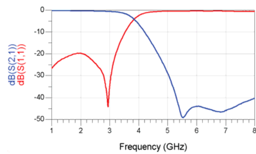
RFLPF16082G6W0T
