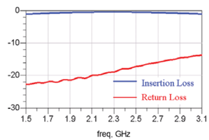
Insertion and Return Loss
