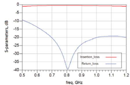
Insertion and Return Loss
