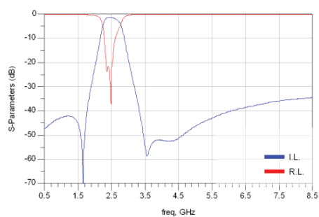
RFBPF1608060AA7M1U
