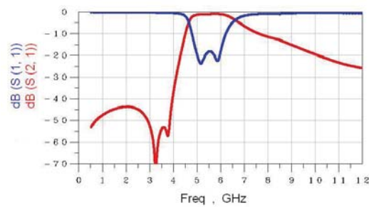
RFBPF2012090K9T
