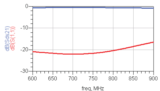
Insertion and Return Loss
