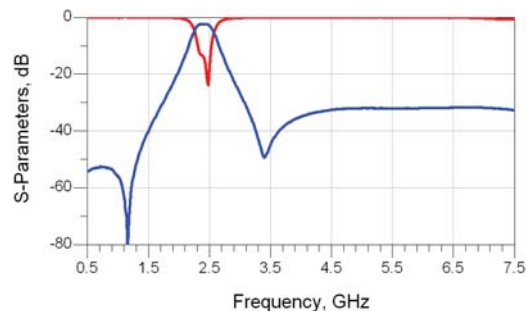
RFBPF1608060A7T
