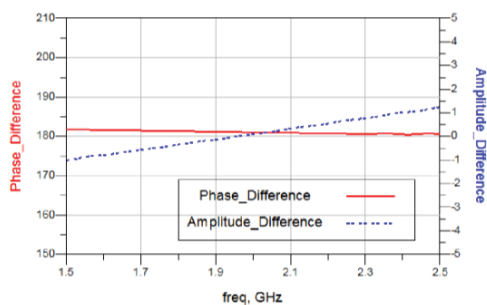
Amplitude and Phase Balance
