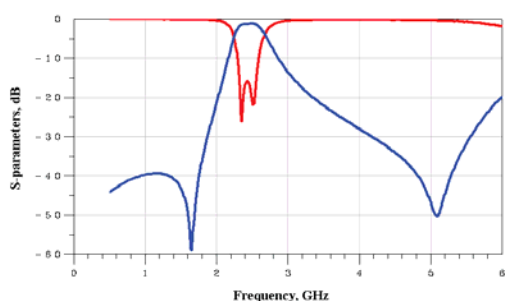
RFBPF2012090A1T
