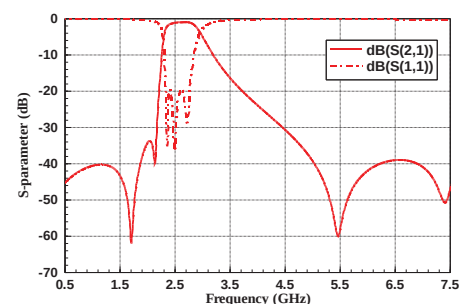
RFBPF2012090ART
