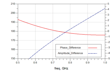
Amplitude and Phase Balance
