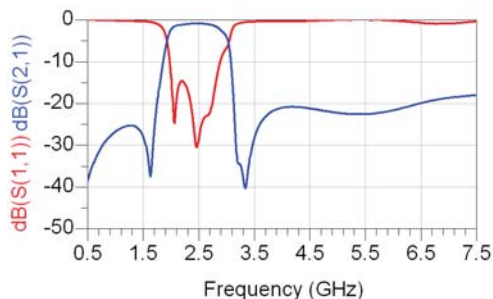
RFBPF2012100AVT
