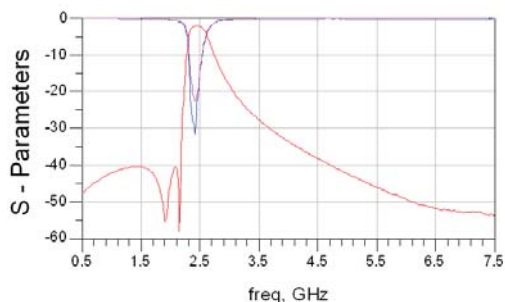
RFBPF2012090AQT
