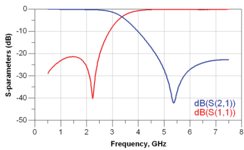
RFLPF1005040A2T
