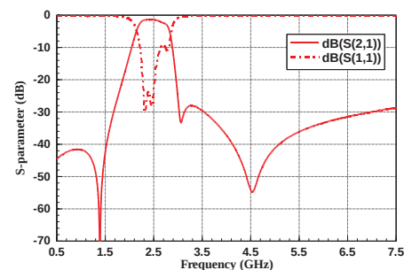
RFBPF1608070AWT
