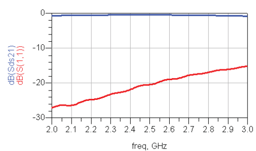
Insertion and Return Loss
