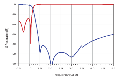
RFLPF10050G9DM1T76
