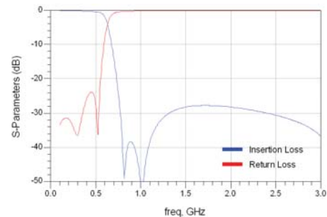
RFLPF2012090Y2T
