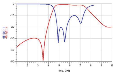
RFBPF2012100K3T
