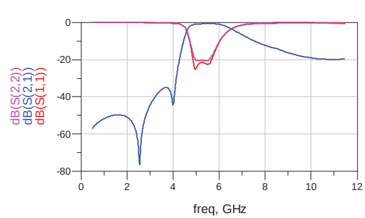
RFBPF1411070E0T
