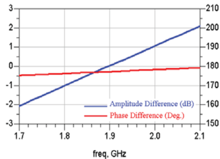
Amplitude and Phase Balance
