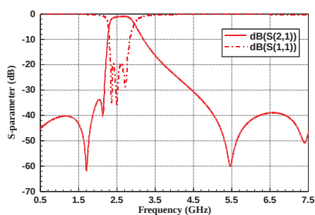
RFBPF2012090A1T
