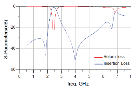
RFBPF2012090A2T
