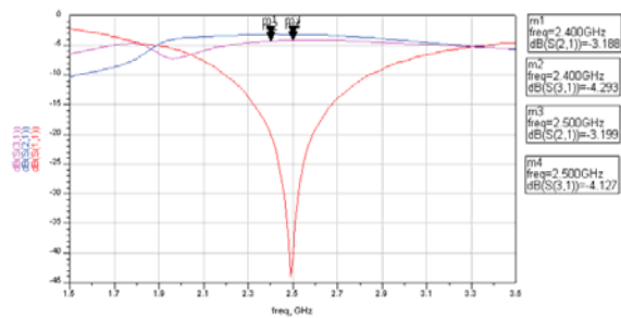
Amplitude and Phase Balance
