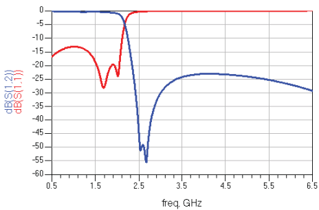
RFLPF1005040A0T
