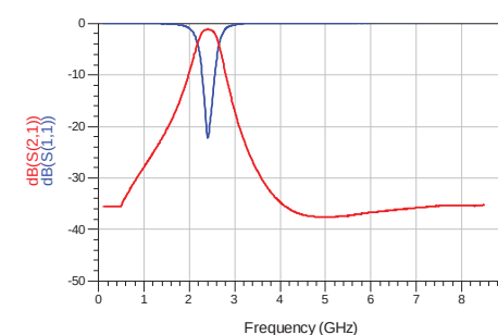
RFBPF1608070AFT
