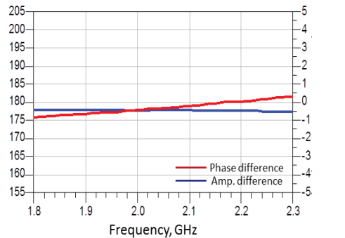
Amplitude and Phase Balance
