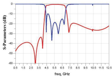
RFBPF2012100KST
