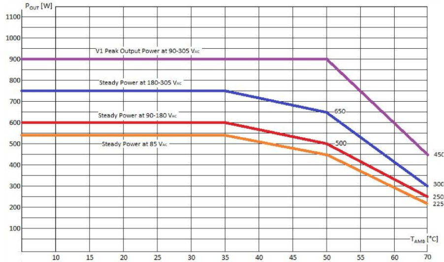
Figure 1 Derating Curves of MCC750 Series V1 P_{OUT} to T_{AMB}
