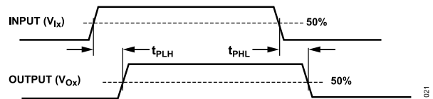
Figure 21. Propagation Delay Parameters
