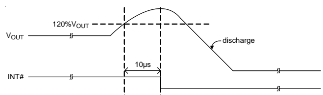
Figure 19. OVP Behavior
