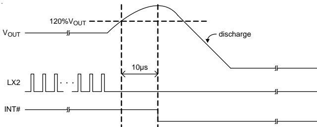
Figure 9. OVP Behavior
