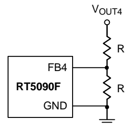
Figure 18. Output Voltage Setting
