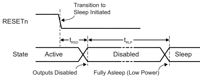
Figure 3a: Transition to Sleep (RESETrn)
