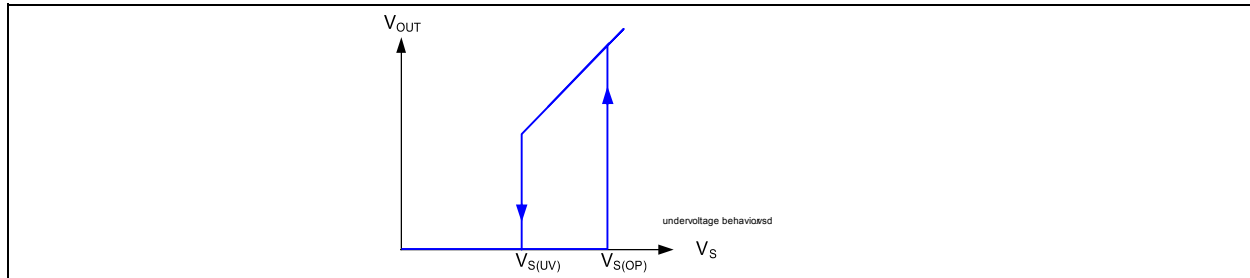
Figure 15 Undervoltage Behavior
