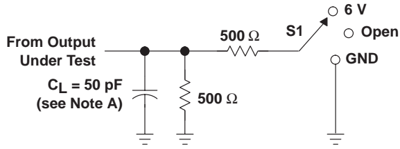
LOAD CIRCUIT
