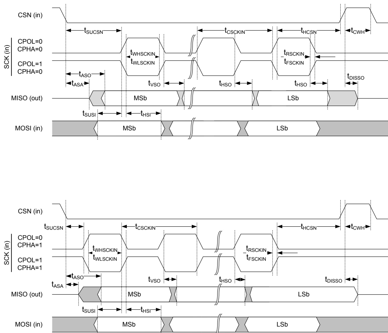
Figure 151: SPIS timing diagram
