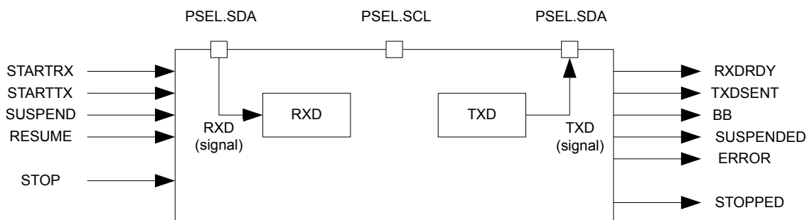
Figure 153: TWI master's main features
