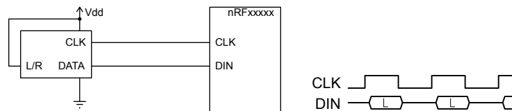
Figure 70: Example of a single PDM microphone, wired as left
