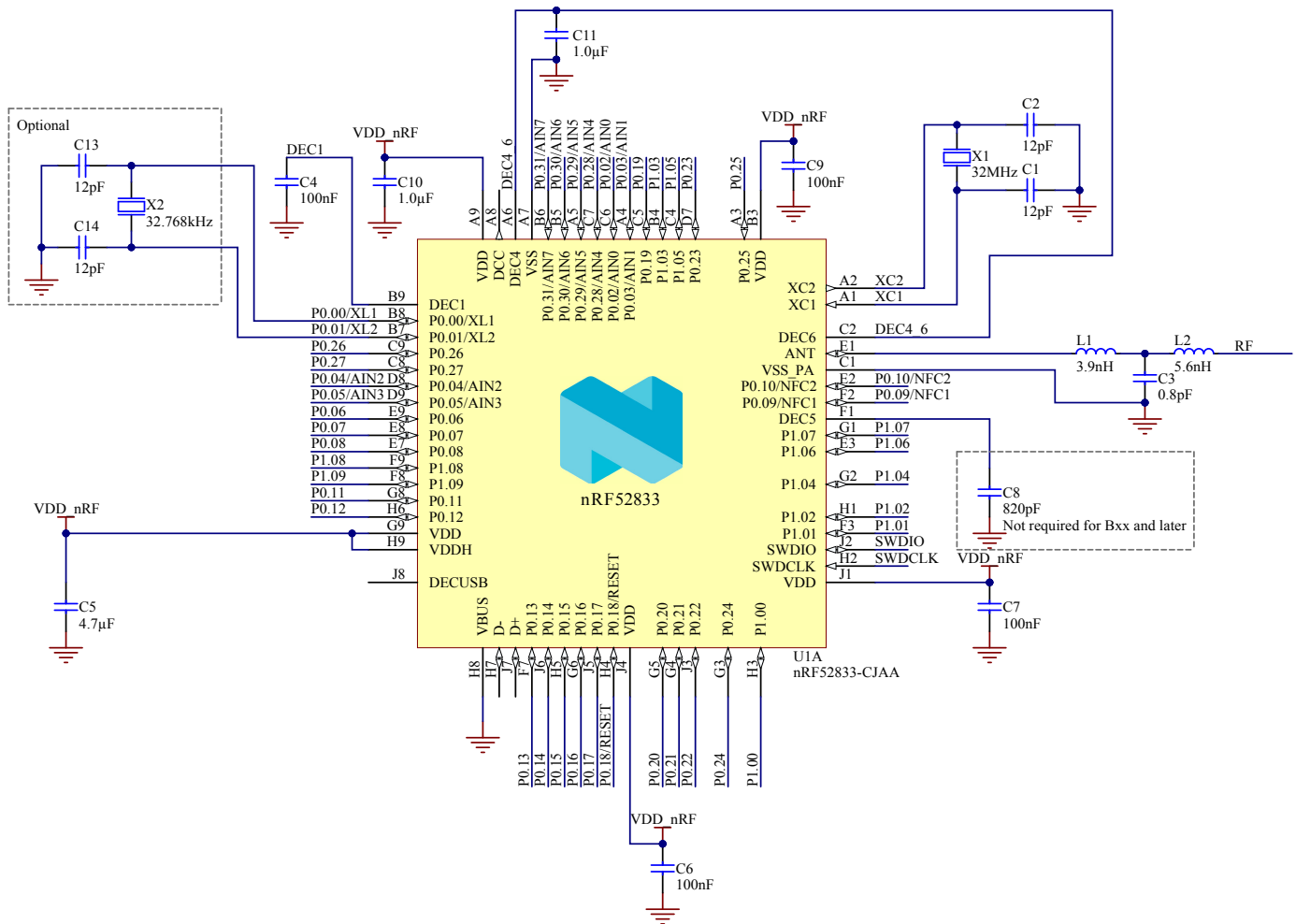
Figure 217: Circuit configuration no. 6 schematic for CJAA WLCSP
