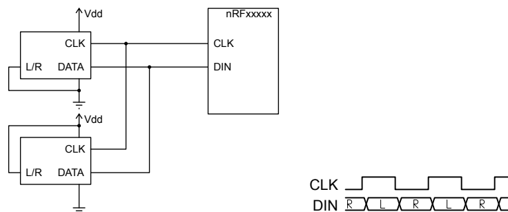
Figure 72: Example of two PDM microphones
