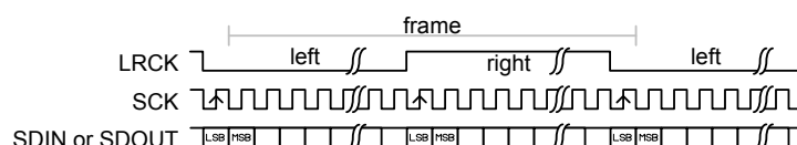
Figure 49: I^2S format. CONFIG.SWIDTH equalling half-frame size.
