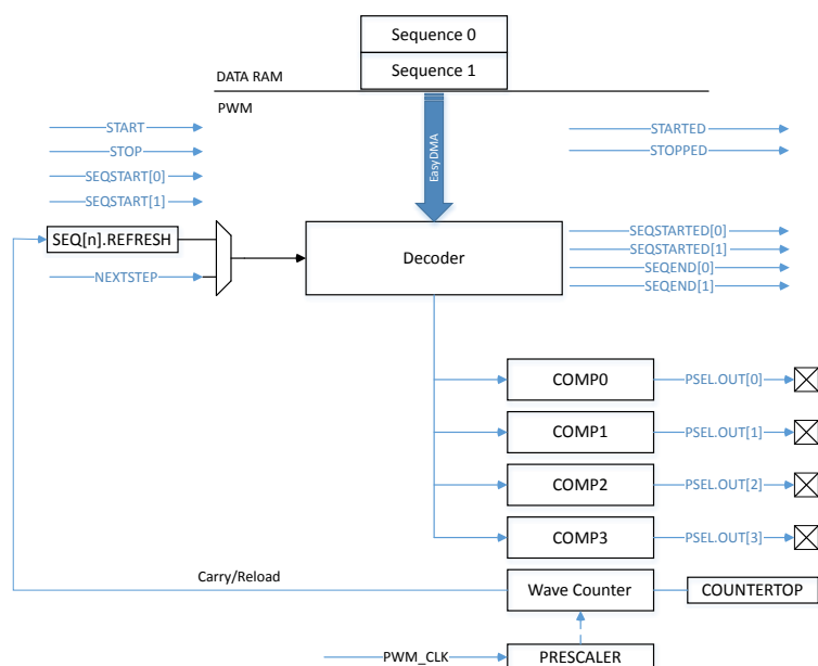
Figure 75: PWM module
