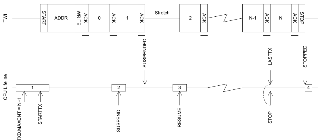
Figure 162: TWI master writing data to a slave
