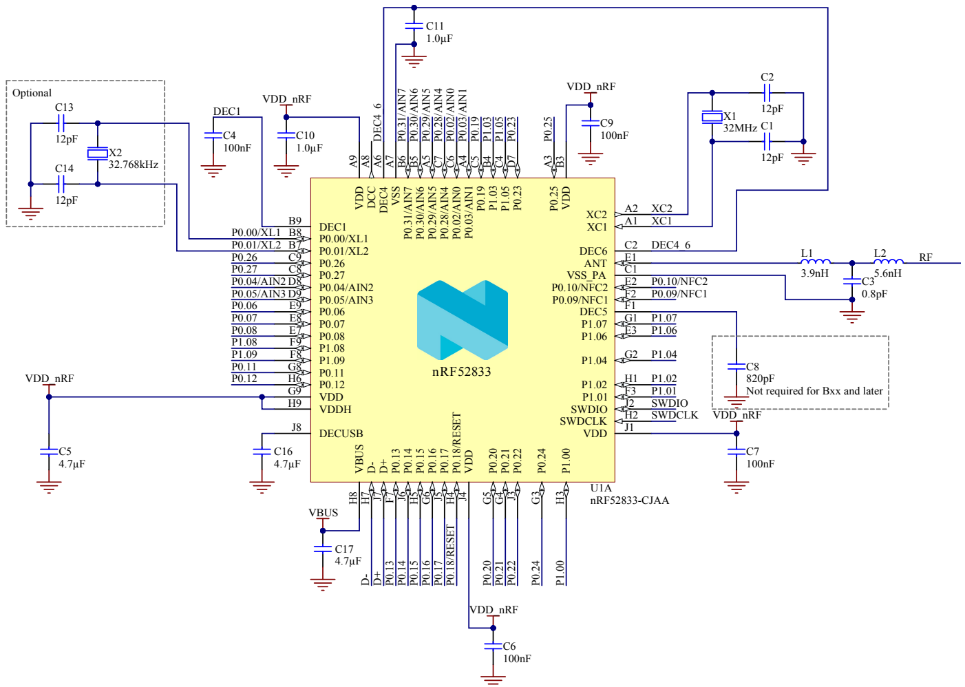
Figure 214: Circuit configuration no. 3 schematic for CJAA WLCSP
