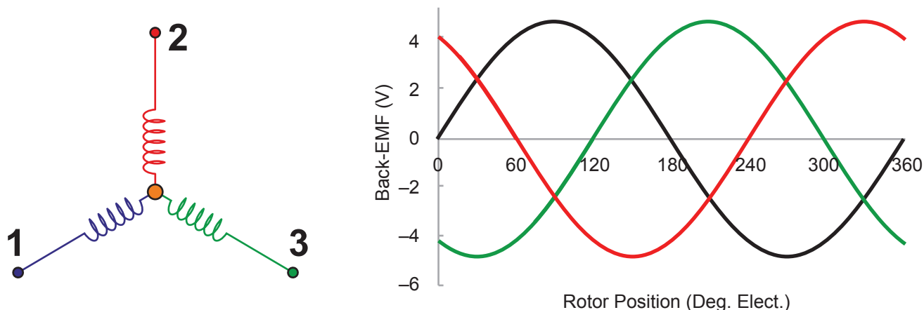
Back-EMF Frequency and Amplitude \propto motor RPM. (Motor BEMF frequency and amplitude are both proportional to motor RPM.)
