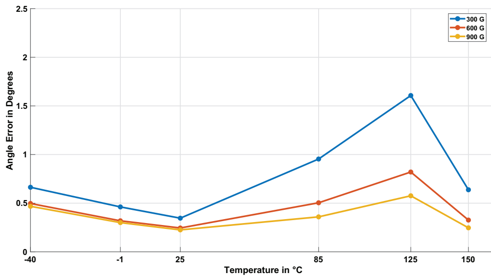
Figure 11: Average Angle Error over Temperature Across 10 Devices. Recommended operating range: 300 G and above.
