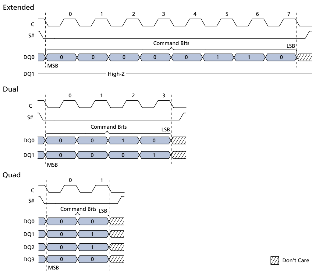
Figure 24: WRITE ENABLE and WRITE DISABLE Command Sequence
