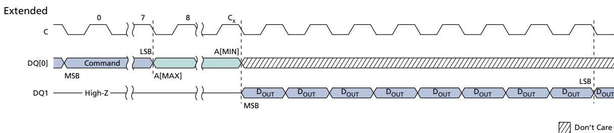
Figure 13: READ Command
