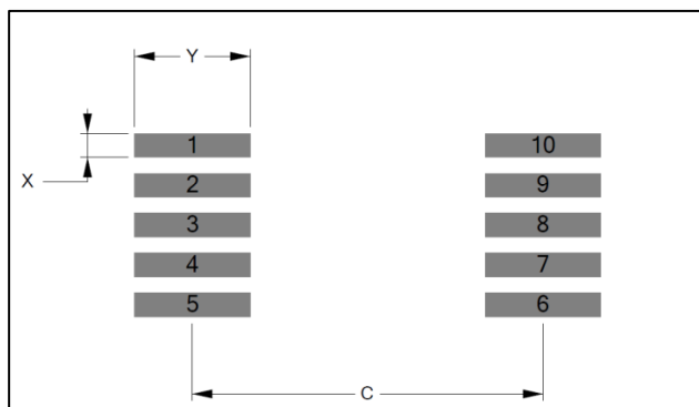
Figure 12.2 MSOP-10 PCB Footprint
