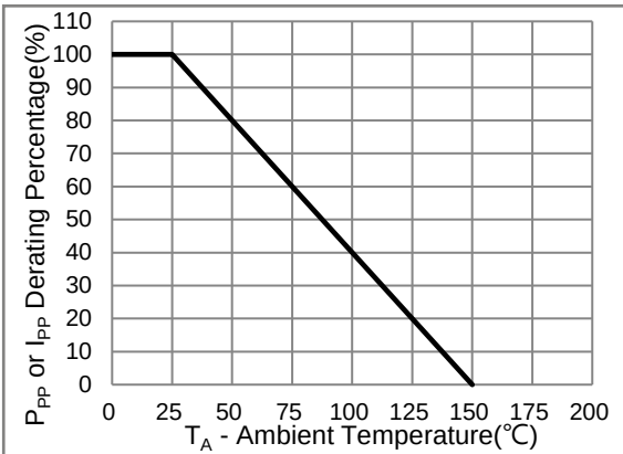
Fig.2 Derating Curve
