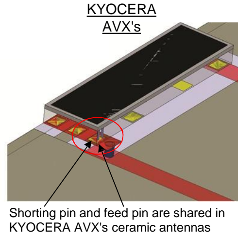
Figure 2 KYOCERA AVX's Antenna Layout (Required)
