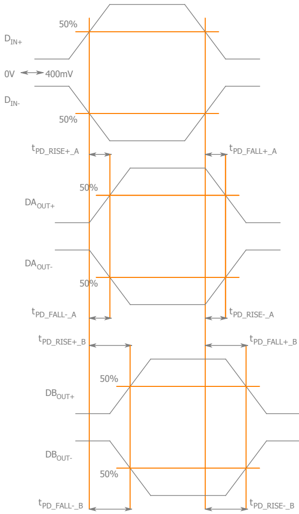
Figure 3. Rise / Fall Propagation Delay & Skew
