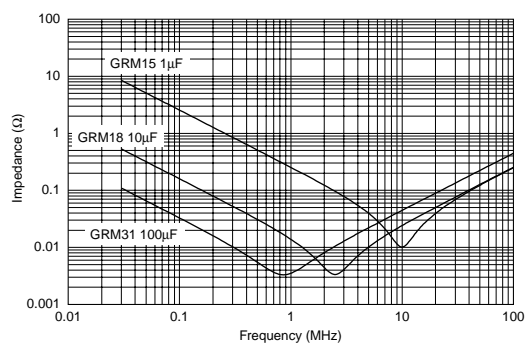
R \Delta
