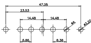
CODE:5W5 MALE
