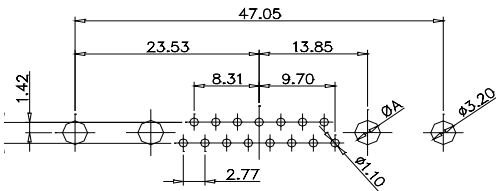
CODE:17W2 MALE/FEMALE
