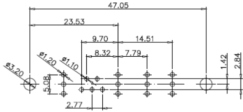
9W4 Female
