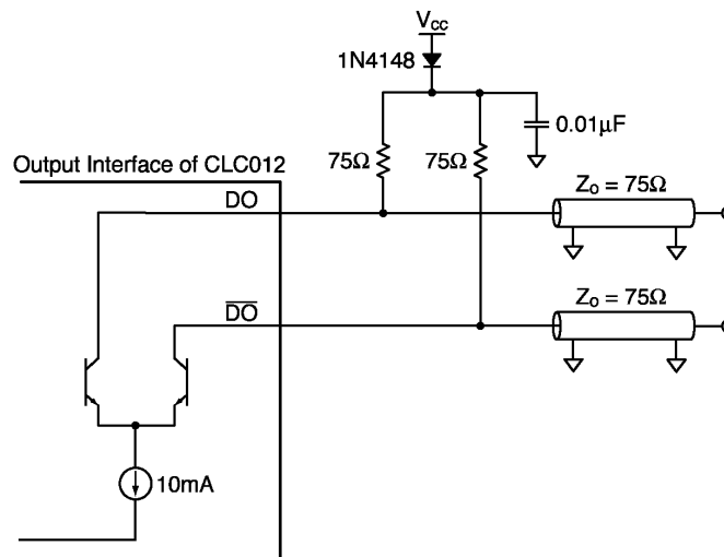
Figure 25. Differential Source Terminated Output Interface
