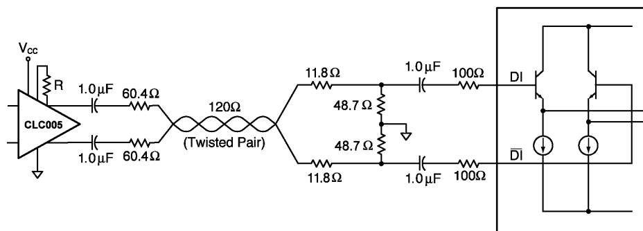
Figure 32. Twisted Pair Equalization
