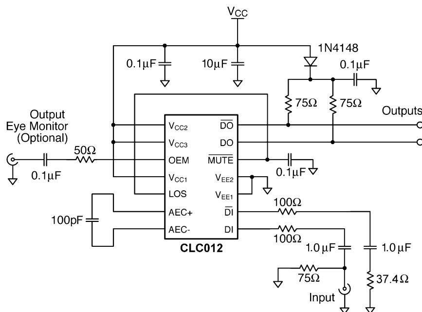
Figure 20. CLC012 Equalizer Application Circuit
