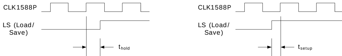
Figure 89 • Load/Save AC Timing
