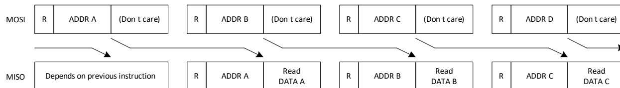
Figure 71 • SPI Multiple Register Reads
