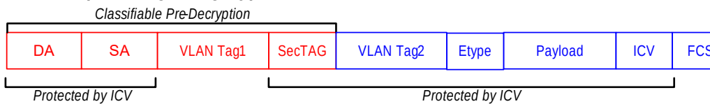
Figure 31 • MACsec Transform to Single and Dual Tag Bypass
