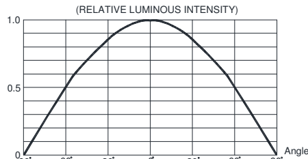
FIG.6 FAR FIELD PATTERN
