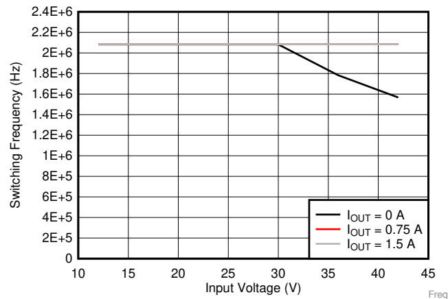
Figure 8-11. Switching Frequency vs Input Voltage V_{OUT} = 5\text{ V}
