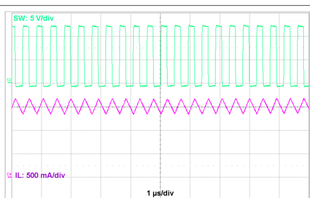
Figure 8-8. Typical PWM Switching Waveforms V_{IN} = 12\text{ V} , V_{OUT} = 5\text{ V} , I_{OUT} = 1.5\text{ A} , f_S = 2100\text{ kHz}
