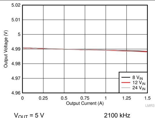
Figure 9-6. Load Regulation
