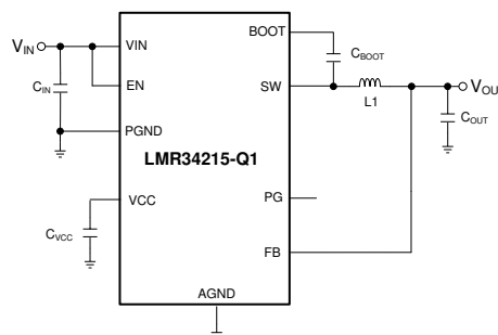
Simplified Schematic
