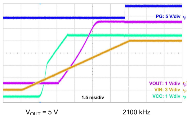
Figure 9-9. Start-Up Waveform
