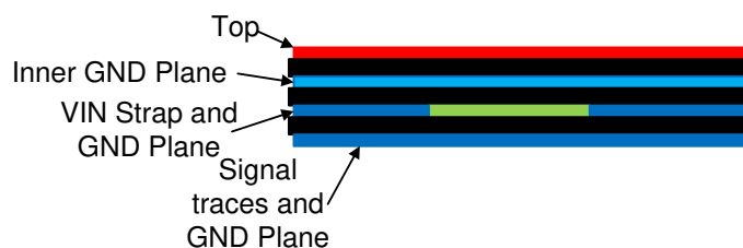
Figure 10-2. Example Layout for Fixed Output
