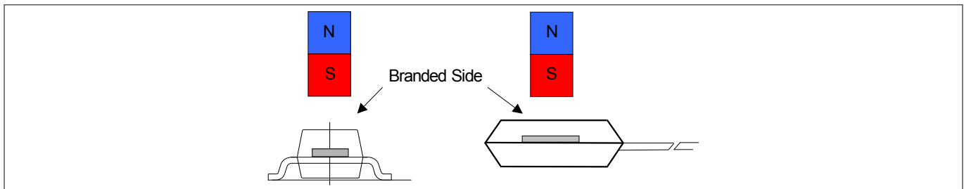
Figure 9 Definition of magnetic field direction PG-SOT23-3-15 (left hand) and PG-SSO-3-2 (right hand)
