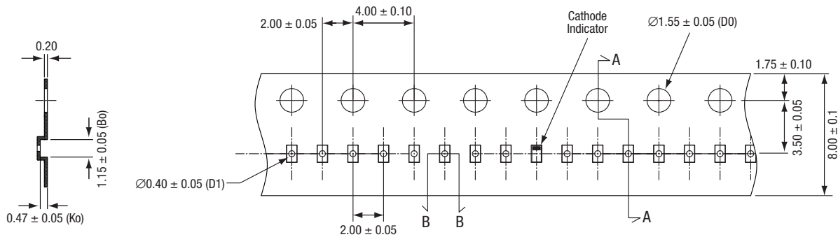
Figure 14. SOD-882 Package Dimensions
