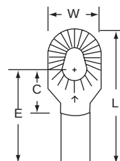
13-610-W Stud Size 6, 8, 10 Wire Range 12-10
