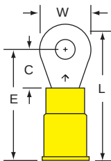
13-6-NB Stud Size 6 Wire Range 12-10
