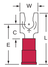
SS-31-8-P 8 22-18
