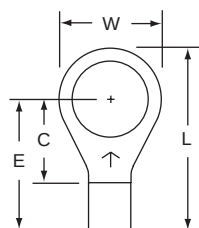
13-56S-W 5/16 12-10
