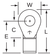
123-8-W 8 16-12
