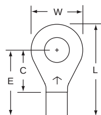
13-14S-W 1/4 12-10
