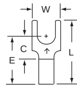
BS-32-10-W
