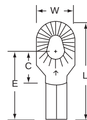
13-610 Stud Size 6, 8, 10 Wire Range 12-10
