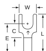
BS-31-10-W
