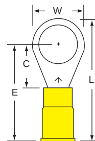
13-38S-P 3/8 12-10
