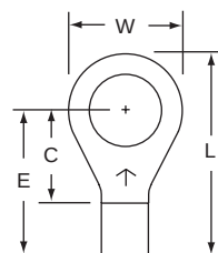
13-38S-W 3/8 12-10
