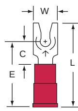
SS-31-4-P 4 22-18
