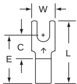
BS-32-6S-W
