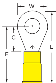
13-14S-P, 1/4 12-10
