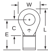
123-10-W 10 16-12
