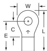
13-6-W 6 12-10
