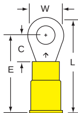
13-10-NB Stud Size 10 Wire Range 12-10
