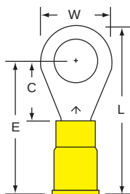
13-56S-P 5/16 12-10
