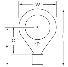
123-500-W 1/2 16-12
