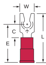
SS-31-6-P 6 22-18
