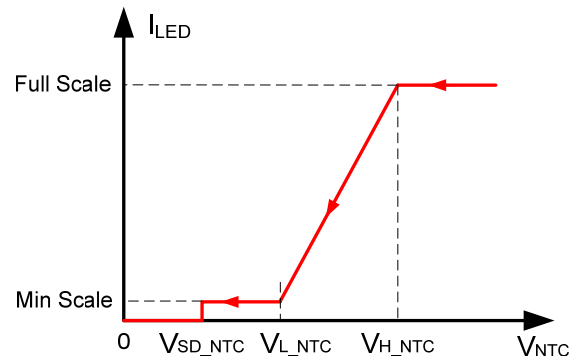
Figure 4: NTC Curve
