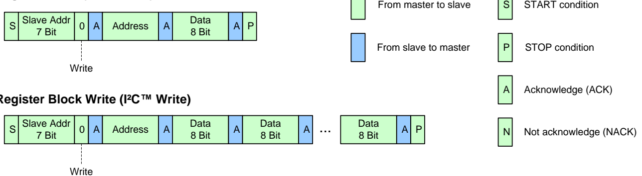
Figure 3.7 I 2 C Register Write
