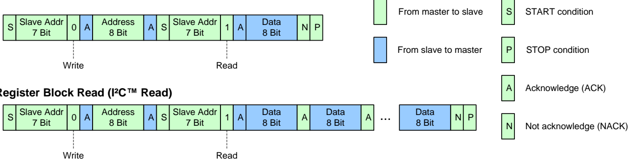
Figure 3.6 I 2 C Register Read
