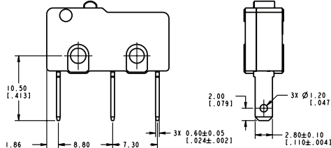
Terminal Type 70 - Long Solder
