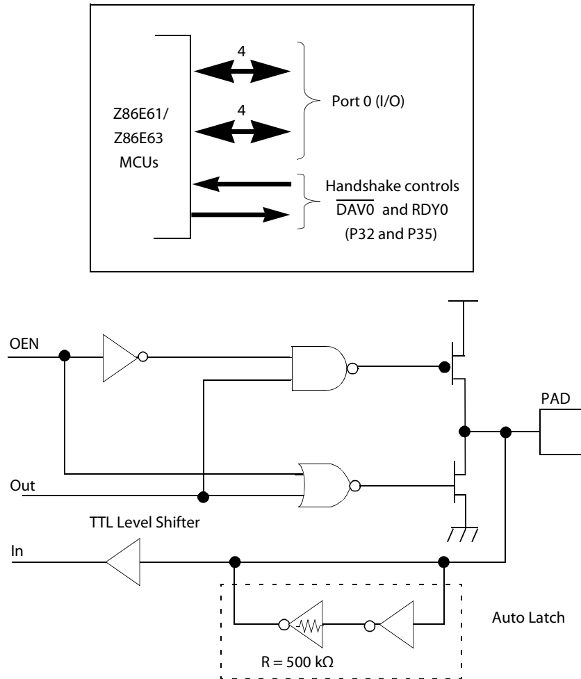
Figure 8. Port 0 Configuration
