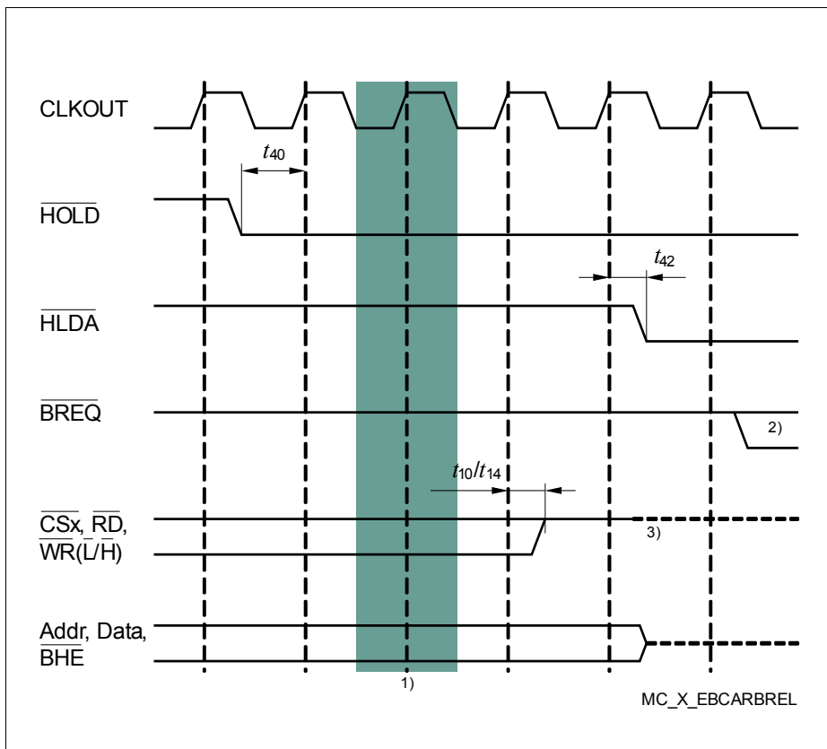
Figure 26 External Bus Arbitration, Releasing the Bus
