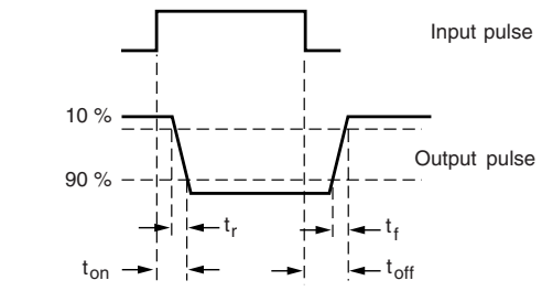
Fig. 3 - Test Circuit and Waveforms
