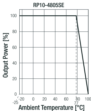
Derating Graph (11)
