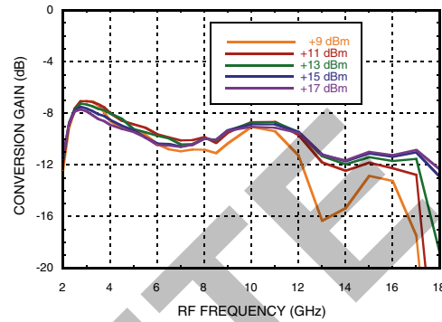
Conversion Gain vs. LO Power, IF = 1500 MHz
