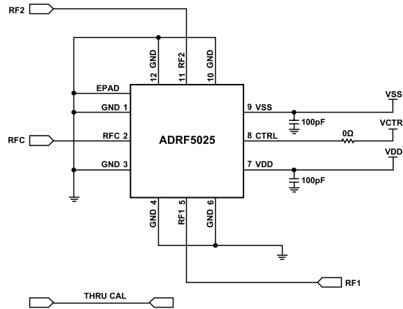
Figure 21. Simplified Evaluation Board Schematic
