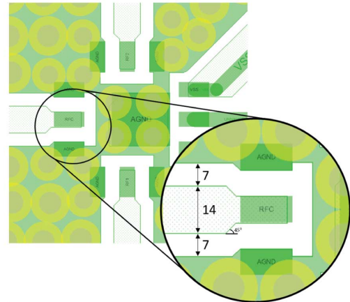
Figure 25. Without Impedance Match
