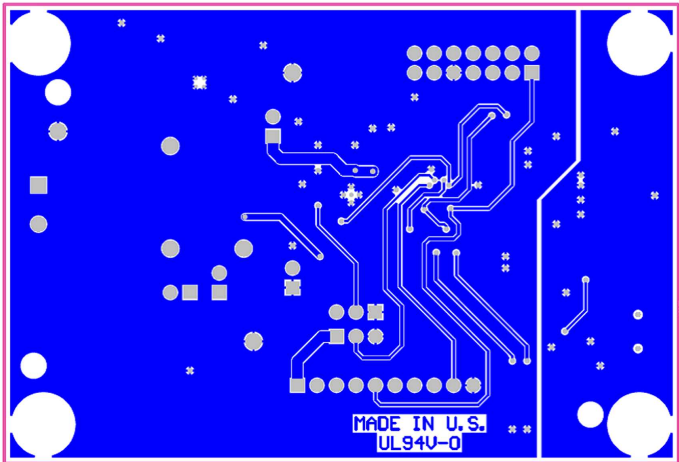
Figure 12. Bottom Layer Routing
