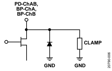
Figure 6. PD-ChAB, BP-ChA, and BP-ChB Interface Schematic
