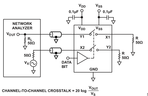
Figure 32. Channel-to-Channel Crosstalk
