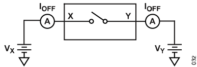
Figure 26. Off Leakage
