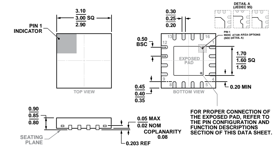
Figure 17. 16-Terminal Lead Frame Chip Scale Package [LFCSP] 3 mm × 3 mm Body and 0.85 mm Package Height (CP-16-50) Dimensions shown in millimeters
