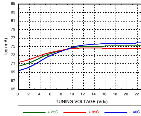
Supply Current
