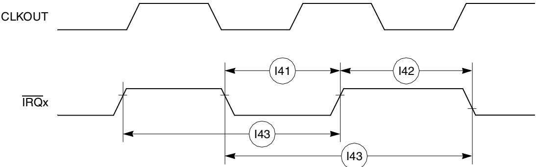
Figure 24. Interrupt Detection Timing for External Edge-Sensitive Lines
