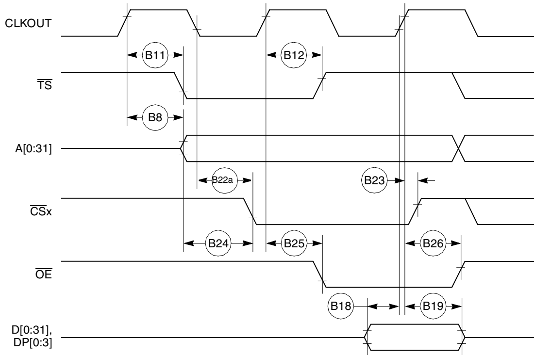
Figure 11. External Bus Read Timing (GPCM Controlled—TRLX = 0, ACS = 10)
