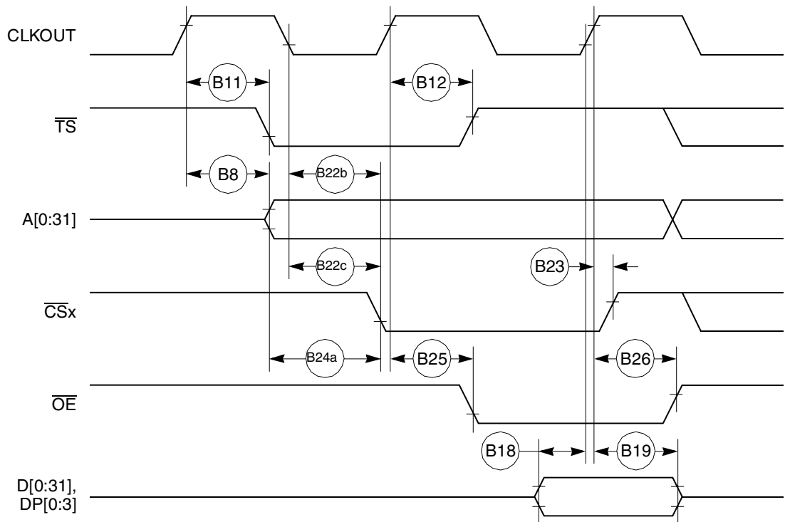
Figure 12. External Bus Read Timing (GPCM Controlled—TRLX = 0, ACS = 11)
