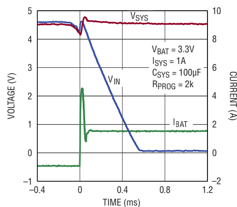
Normal to Backup Mode Transition Waveform
