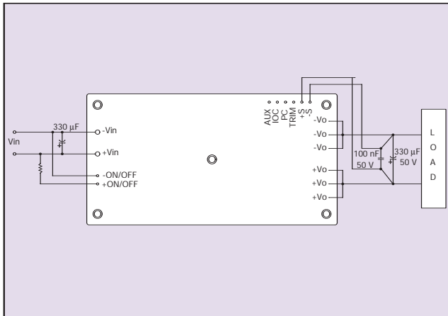
Figure 1 - Standard Application
