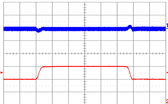
Figure 1.2V.17. Output voltage response to load current step-change (20 A - 30 A - 20 A) at V_{in} = 48\text{ V} . Top trace: output voltage (100 mV/div.). Bottom trace: load current (10 A/div.). Current slew rate: 0.1 A/ \mu\text{s} . C_o = 1\ \mu\text{F} ceramic. Time scale: 0.2 ms/div.
